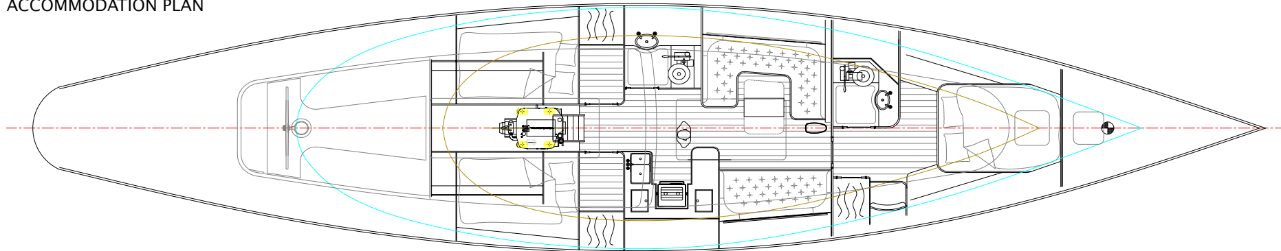
ACCOMMODATION PLAN
